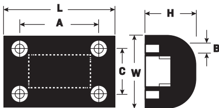
Dimensions are for reference only. Actual dimensions may vary.
