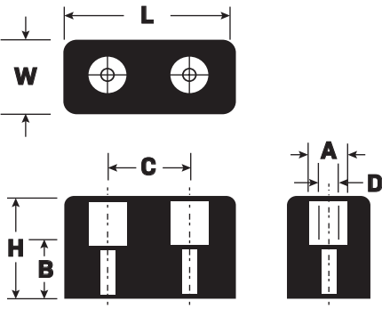
Dimensions are for reference only. Actual dimensions may vary.
